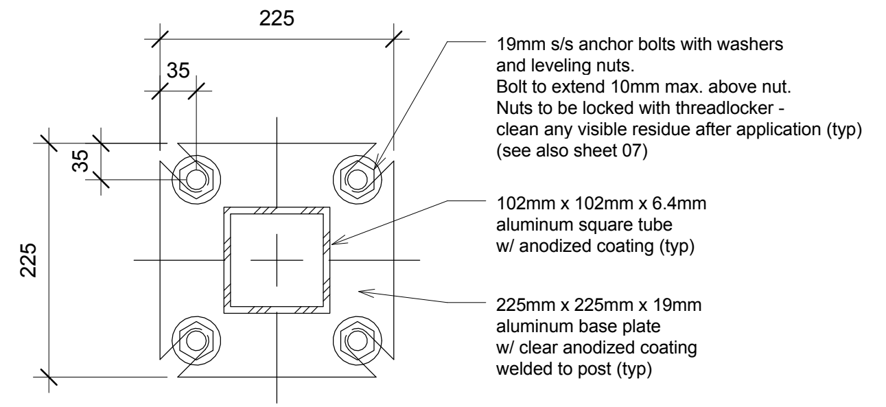
section b (slip base) scale 1:5
